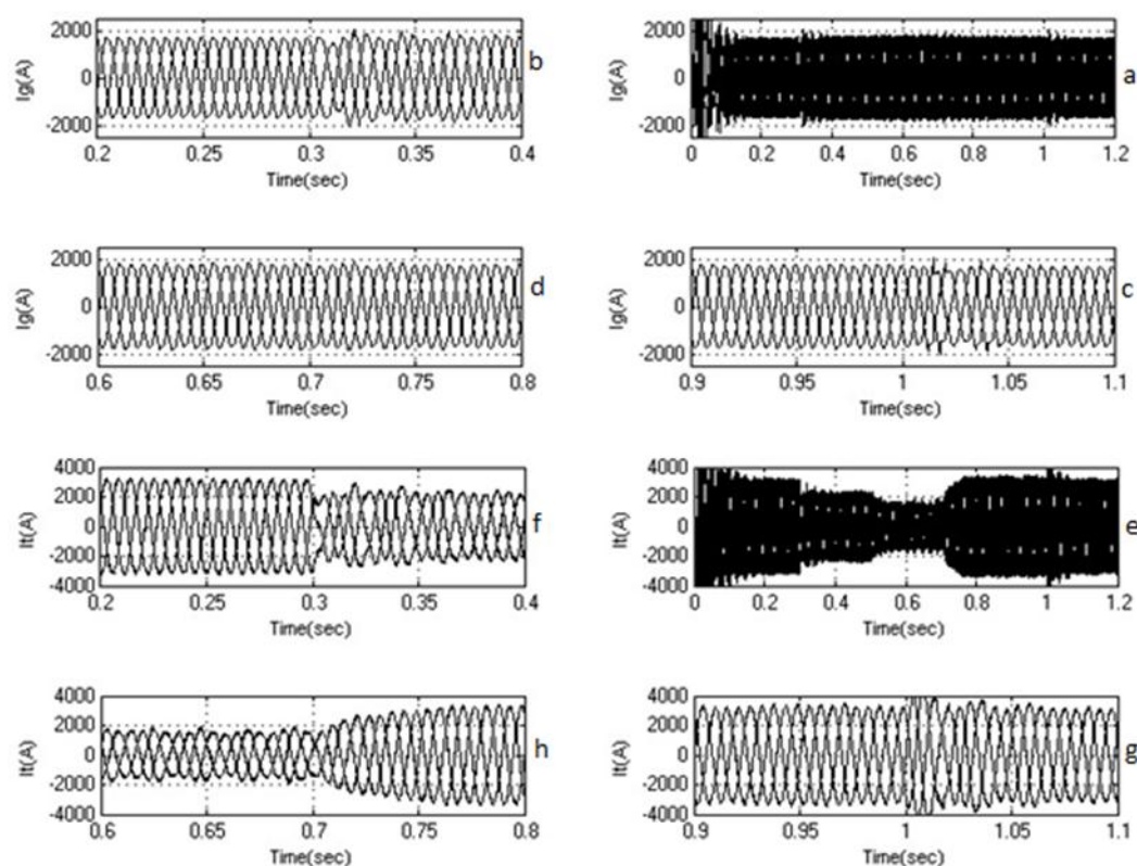
Figure (7): Current of the converter located on the network side during changes in reference of active and reactive powers for machine speed of 2160 RPM at voltage balance mode a) Current of the converter located on the network side b) Upscaling current of the converter located on the network side during change in reference of active power c) Upscaling current of the converter located on the network side during change in reference of active and reactive powers into the primitive mode d) Upscaling current of the converter located on the network side during change in reference of reactive power e) network current f) Upscaling current of the converter located on the network side during change in reference of active power g) Upscaling current of the network during change in reference of active and reactive powers into the primitive mode h) Upscaling current of the network during change in reference of reactive power (t= 0.3 sec. change in reference of active power, t=0.5 sec. change in reference of active power in positive direction, t=0.7 sec. change in reference of active power in negative direction, t= 1 sec. change in reference of active and reactive power into the primitive mode).
