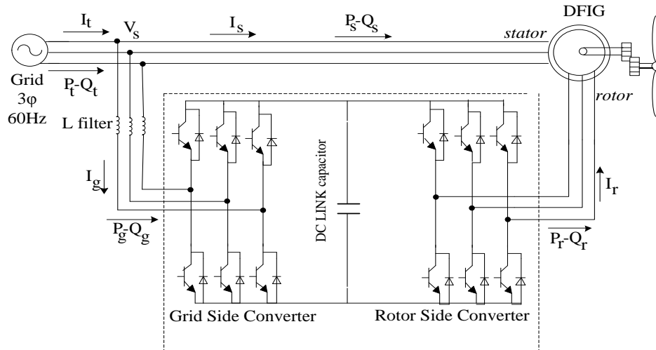
Figure 1: use of converter for injecting power from DFIG into the network schematic design of controller of the converter located on the network side
