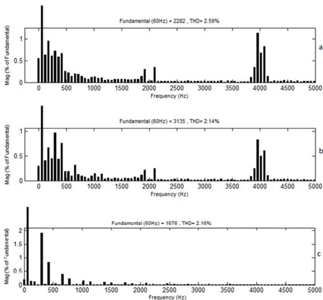
Figure (4): Output current of the simulated system for machine speed of 2160 RPM at voltage balance mode : a) THD of stator current, b) THD of infinite bus current , c) THD of injecting current from the converter located on network side
