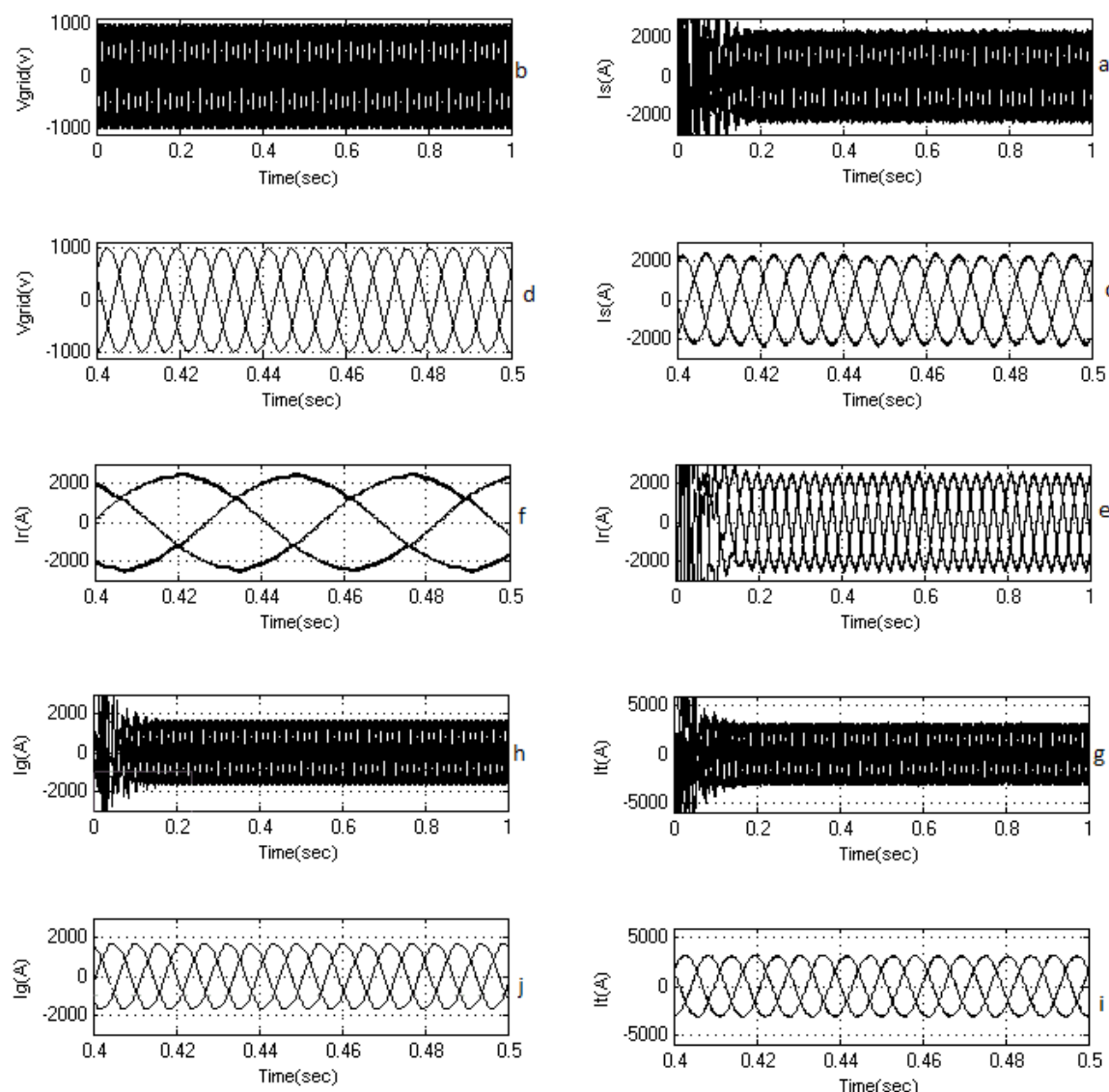
Figure (2): output of the simulated system for machine speed of 2160 RPM at voltage balance condition; a) stator current, b) network voltage, c) Upscaling stator current at permanent mode, d) Upscaling network voltage, e) Rotor current f) Upscaling rotor current, g) infinite bus current, h) current of the converter located on network side, i) Upscaling infinite bus current, j) Upscaling current of the converter located on network side
