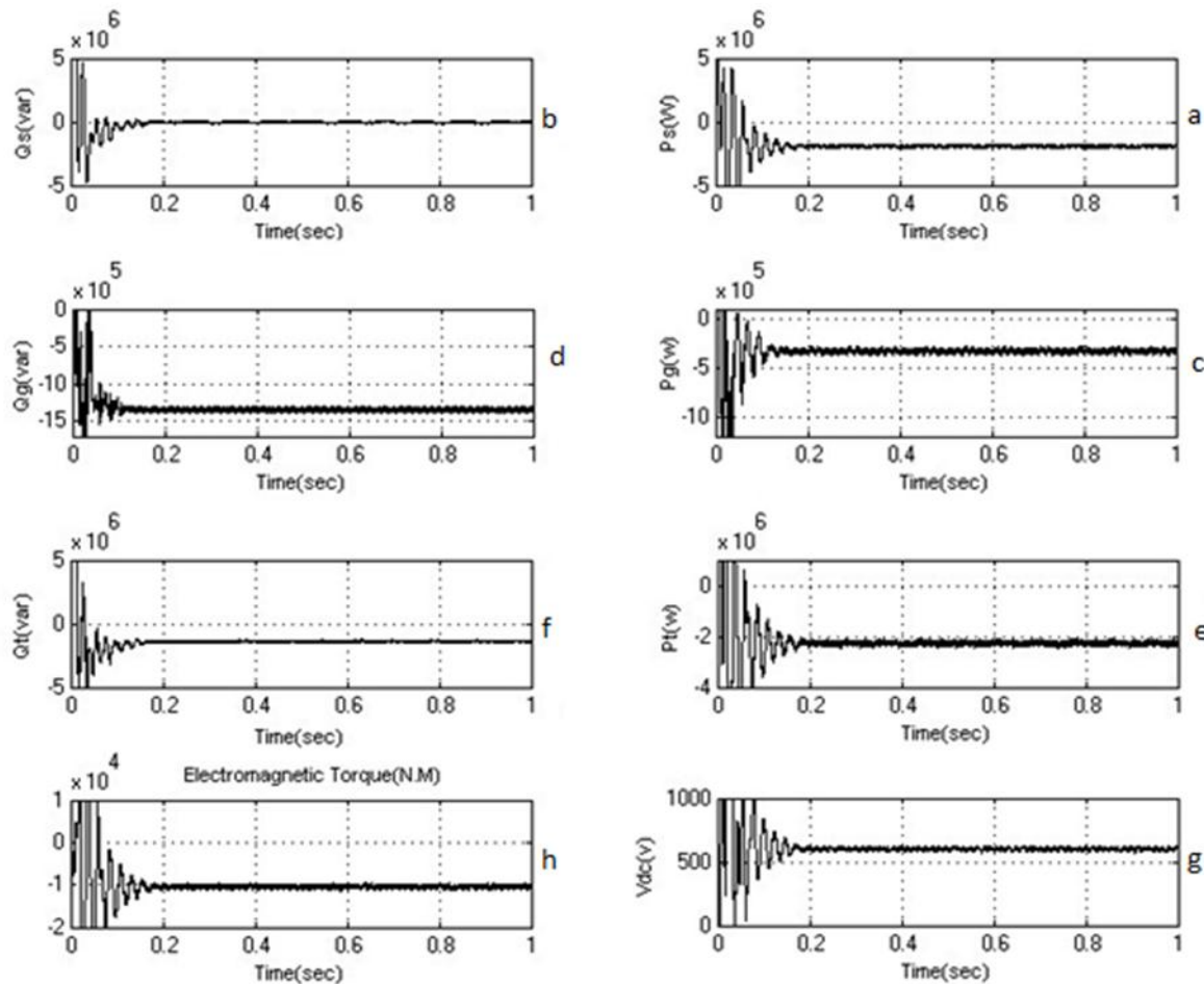
Figure (3): output power of the simulated system for machine speed of 2160 RPM at voltage balance mode a) active power of the stator , b) reactive power of the stator , c) active power of the converter located on network side , d) reactive power of the converter located on network side , e) active power of infinite bus , f) reactive power of infinite bus , g) DC link voltage , h) Electromagnetic Torque
