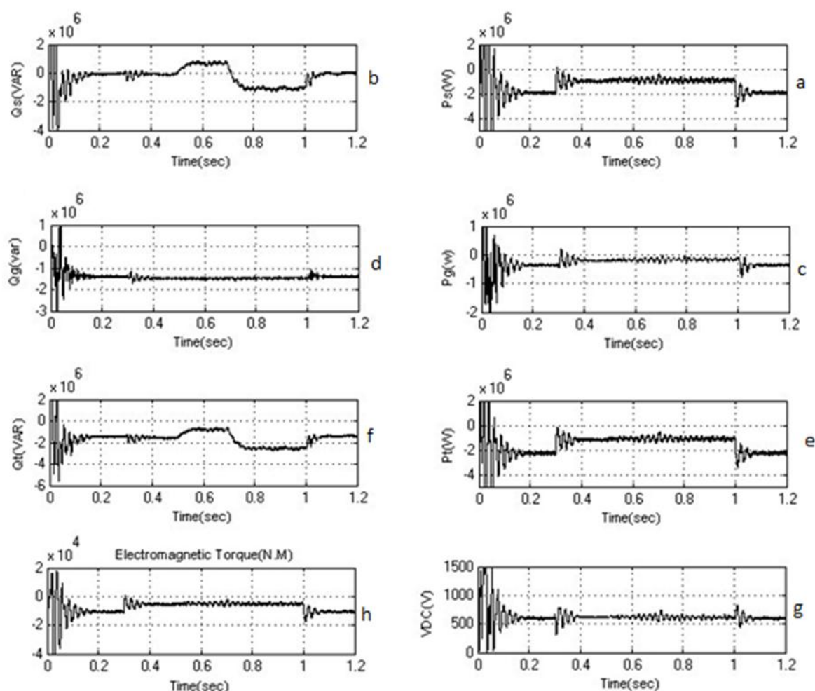
Figure (5): Controllability of output power of the simulated system for machine speed of 2160 RPM at voltage balance mode: a) active power of the stator , b) reactive power of the stator , c) active power of the converter located on network side , d) reactive power of the converter located on network side , e) active power of infinite bus , f) reactive power of infinite bus , g) DC link voltage , h) Electromagnetic Torque (t= 0.3 sec. change in reference of active power, t=0.5 sec. change in reference of active power in positive direction, t=0.7 sec. change in reference of active power in negative direction, t= 1 sec. change in reference of active and reactive power into the primitive mode).
