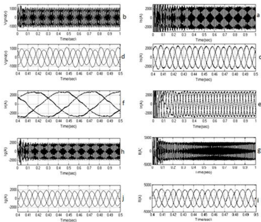
Figure (8): output of the simulated system for machine speed of 2160 RPM at voltage imbalance mode: a) stator current , b) network voltage , c) Upscaling of stator current at permanent mode d) Upscaling of network voltage e) rotor current f) Upscaling of rotor current g) infinite bus current h) current of the converter located on the network side i) Upscaling of infinite bus current j) Upscaling of current of the converter located on the network side
