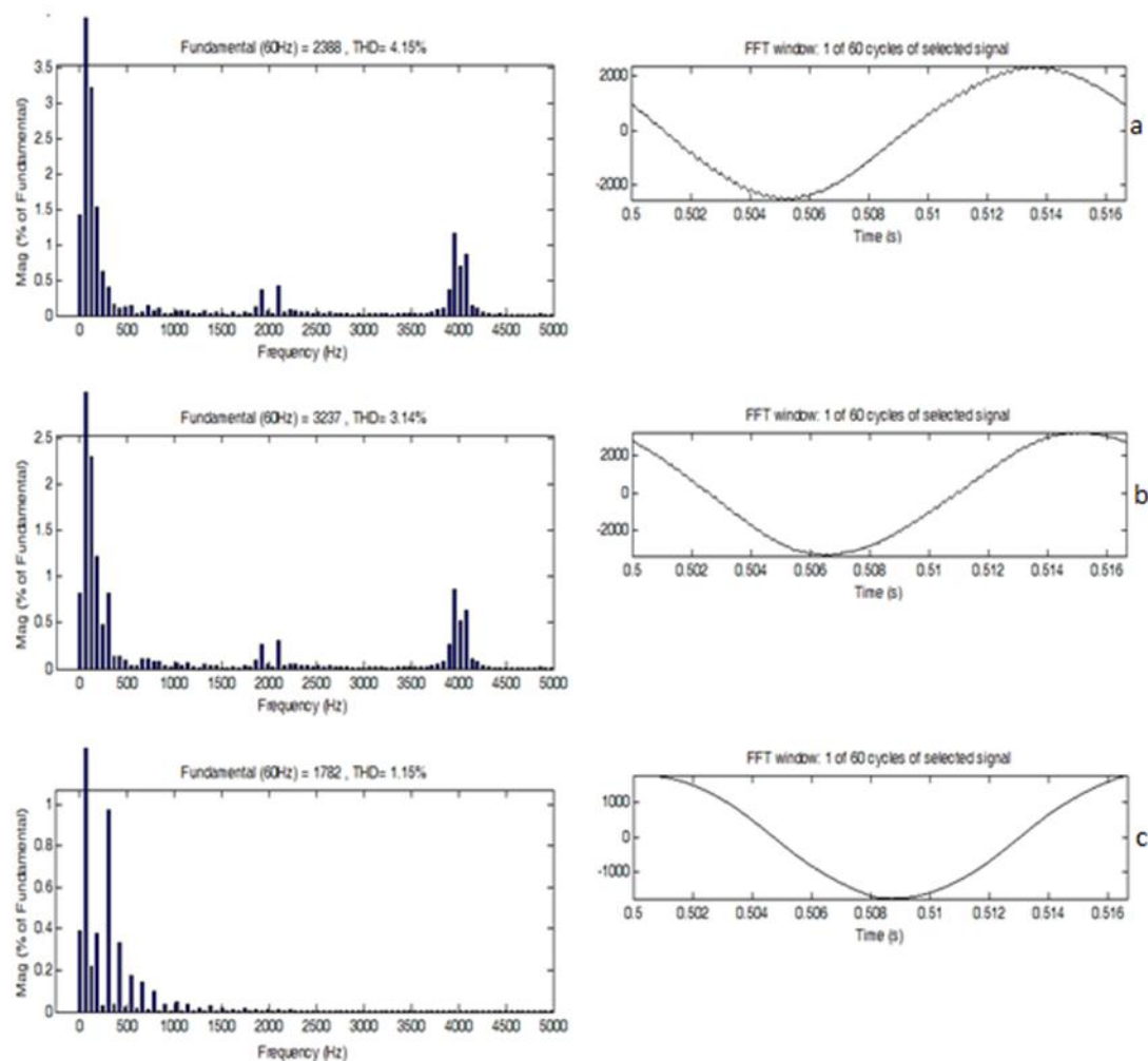
Figure (10): output current of the simulated system for machine speed of 2160 RPM at voltage imbalance condition; a) THD of infinite bus current b) THD of the current injected from the converter located on network side c) THD of the stator current
