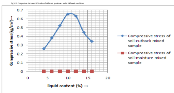
Fig 3 UCS value of different specimens under different conditions
