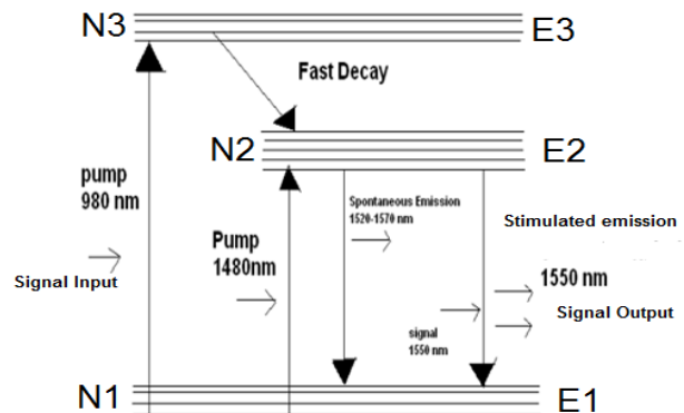
Figure 3: Erbium doped fiber amplifier Design
