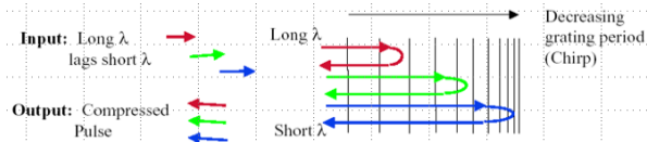
Figure 8: Dispersion Compensation
