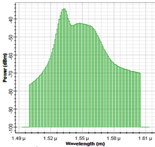
Figure 11: ASE of EDFA
