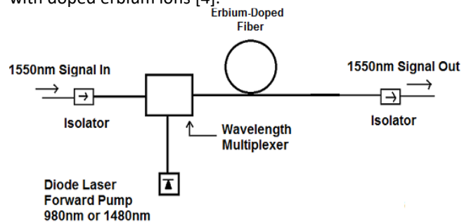
Figure 3: Erbium doped fiber amplifier Design
