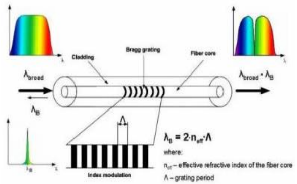
Figure 6: Bragg grating equation
