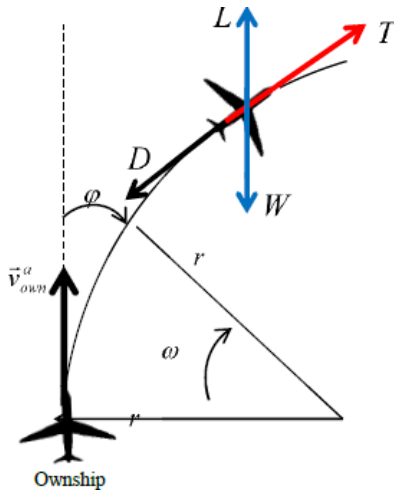
Figure 2: Top view of a turning flight in a horizontal plane The tangential acceleration ( \underline{a} ) of the airborne aircraft can be written as the derivative of two functions,
