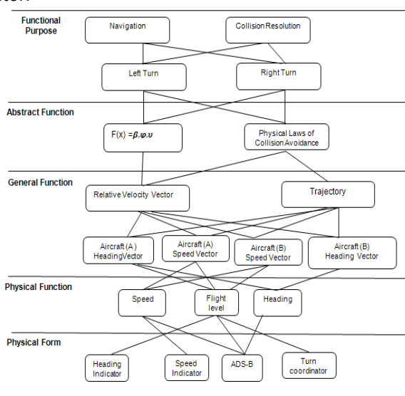
Figure 3: Abstraction Hierarchy of Flight Collision Avoidance display
