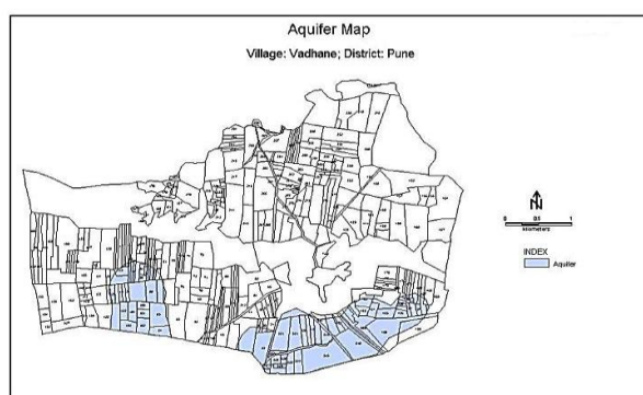
Fig. 6: Aquifer map of Village Vadhane
