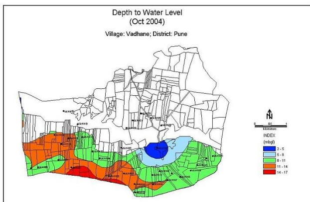
Fig. 3: Depth to water level for Post monsoon period.
