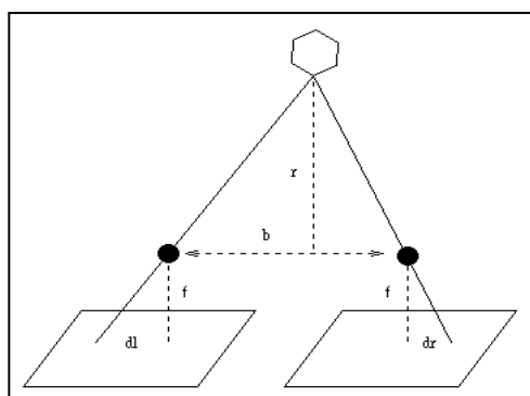
Figure 5: Stereo geometry
