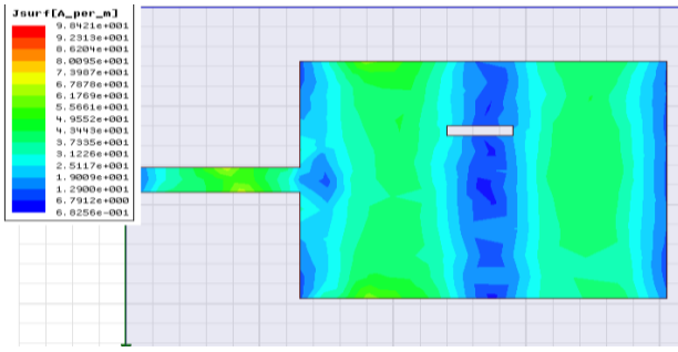
Fig.5 Current distribution after placing slot
