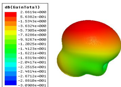
Fig.11 Gain of antenna after placing slot1 at 25mm and slot2 at 28mm
