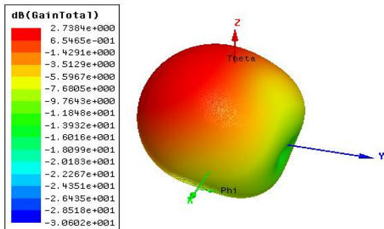
Fig. 7 Gain after three slots
