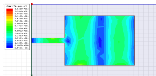
Fig.4 Current distribution at 5GHz
