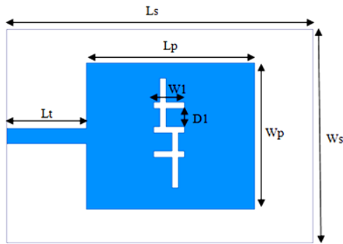
Fig.1 Antenna geometry
