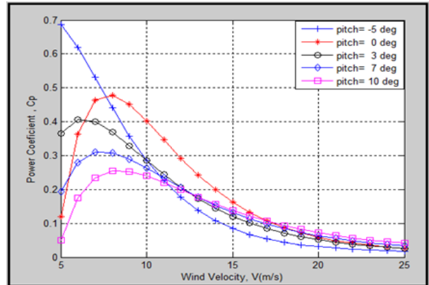
Figure (6) : Relationship between Power coefficient and wind Velocity for different pitch angles
