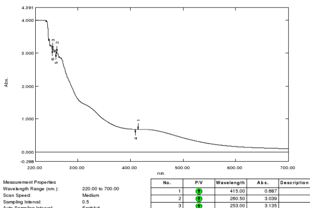
Fig. 3: UV spectrum of Ag nanoparticles obtained by 3mM AgNO 3 and Lemon extract
