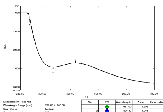
Fig. 1: UV spectrum of Ag nanoparticles obtained by 1mM \text{AgNO}_3 and Lemon extract
