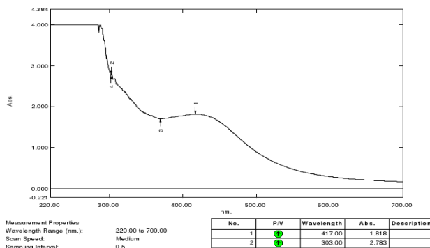
Fig. 5: UV spectrum of Ag nanoparticles obtained by 4mM AgNO 3 and Lemon extract
