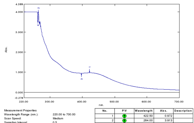
Fig. 4: UV spectrum of Ag nanoparticles obtained by 4mM AgNO 3 and Lemon extract
