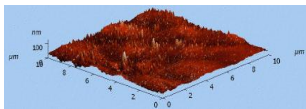
Fig. 6: AFM image of Ag nanoparticles obtained by 5mM AgNO 3 and Lemon extract
