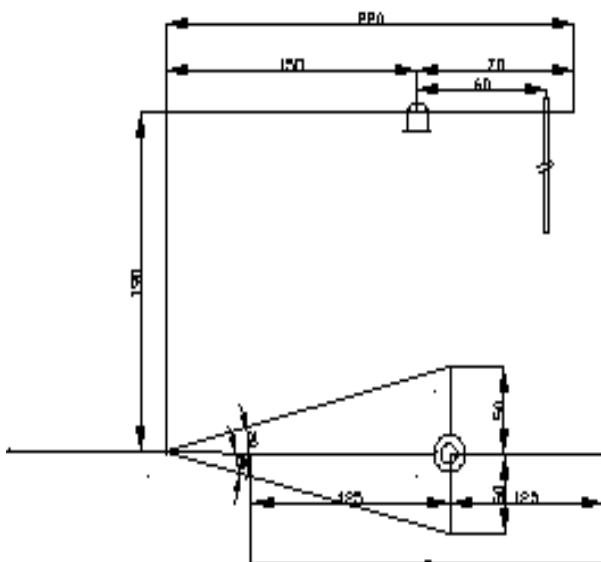
Fig.2 Free body diagram – new clutch pedal Max. Clutch force at top of the pedal = 100N
