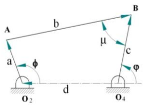
Figure-2 Four bar linkage of 1 st phase.
