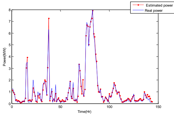
Figure 6 Wind power prediction for the next one day in chester unit by Levenberg-marquardt algorithm
