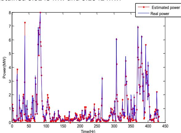
Figure 7 Wind power prediction for the next three days in chester unit by Pso algorithm
