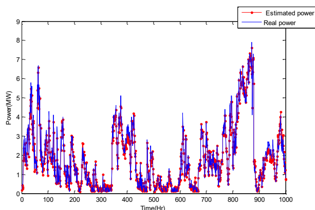
Figure 3 Wind power prediction in small – scale (relating to next seven days) in Stanford unit
