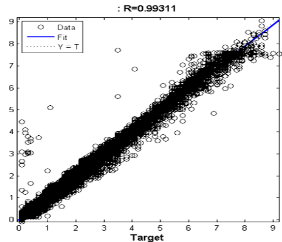
Figure 4 Regression relating to training elman neural network with Pso algorithm
