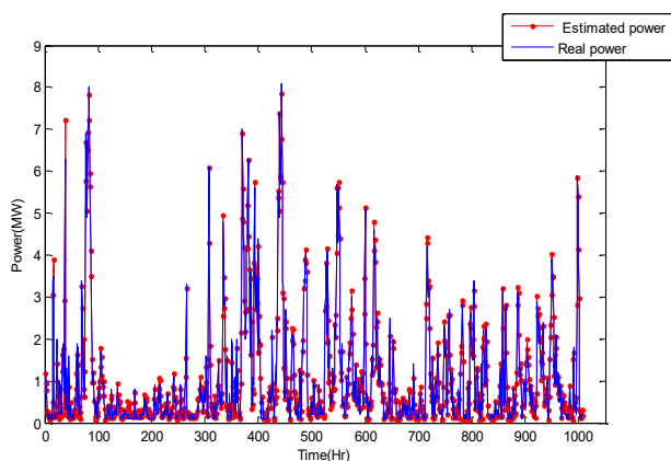
Figure 12 Wind power prediction for the next seven days in chester unit by Levenberg-marquardt algorithm
