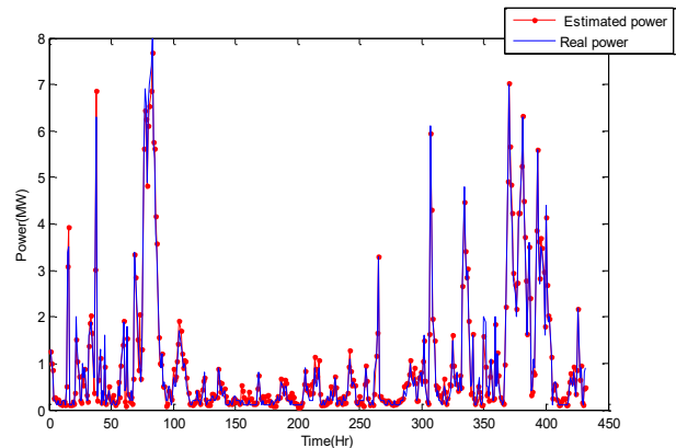
Figure 8 Wind power prediction for the next three days in chester unit by Levenberg-marquardt algorithm
