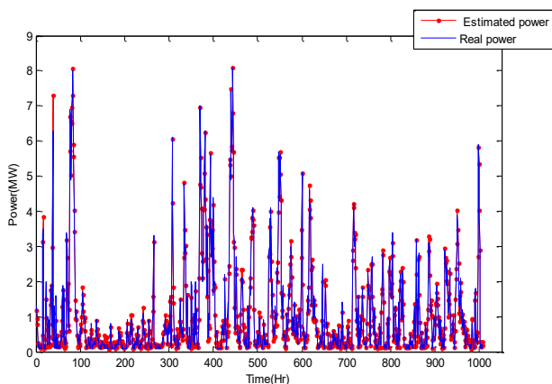
Figure 11 Wind power prediction for the next seven days in chester unit by Pso algorithm
