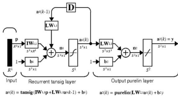
Figure 1 A two-layer Elman network
