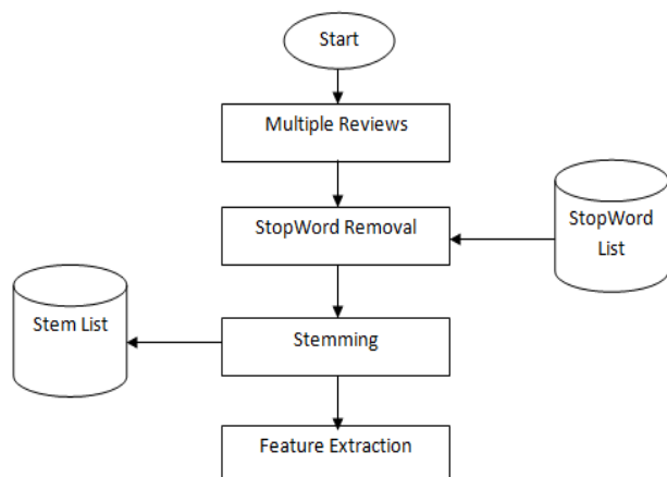
Fig.1 Pre-Processing
