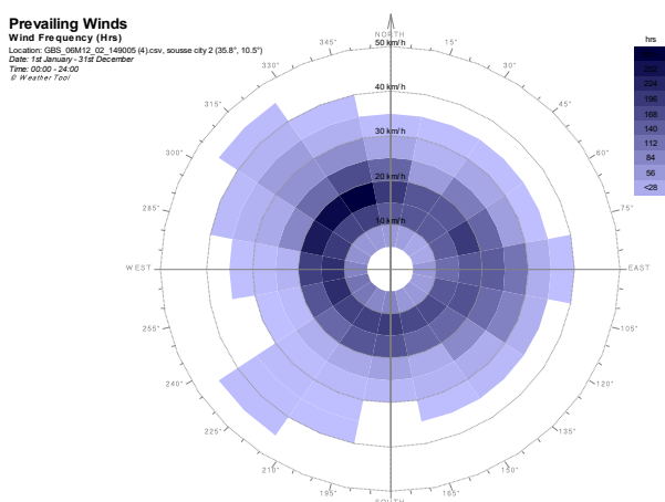
Prevailing annual wind speed using Ecotect Weather Tool
