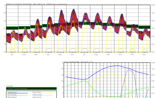
Monthly Diurnal Averages using Ecotect Weather tool
