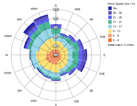
Revit chart annual wind rose
