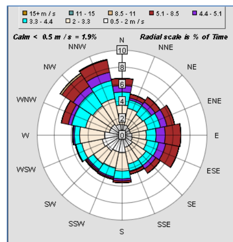
GBS chart annual wind rose
