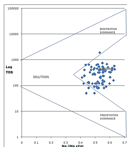
Figure 3: Gibbs Diagram of the Water Sample.
