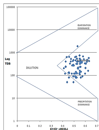
Figure 4: Gibbs Diagram of the Water Sample
