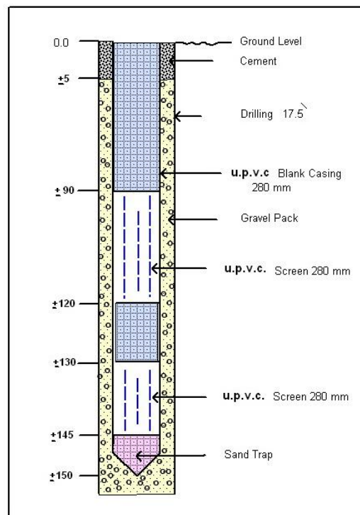
Figure 15: Proposed design for Production well and Injection wells to work in closed system (Injection & Recovery)
