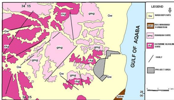
Figure 6: Geological Map of the study area.
