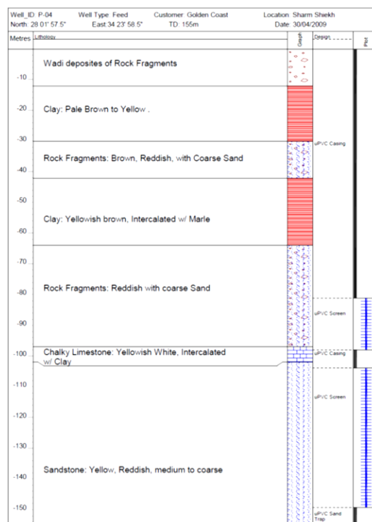
Figure 13: The subsurface lithology distribution in production well no. P4
