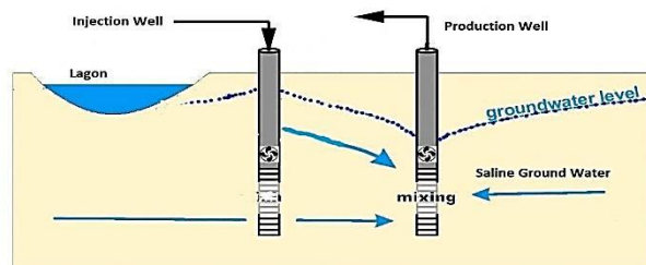
Figure 5: A proposed cross section of the proposed lake showing the mechanism of operation of the feeding and drainage wells in a closed system (the water that is discharged is re-pumped again).
