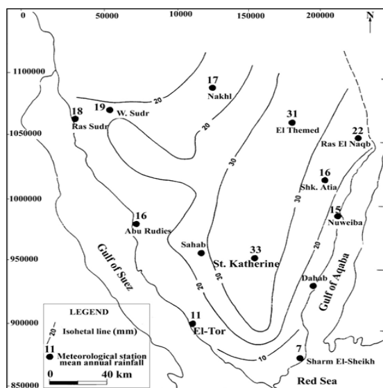
Figure 12: Mean annual rainfall in South Sinai (JICA & WRI, 1999)
