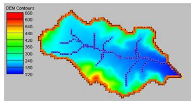
Figure 9: The DEM of the study basin
