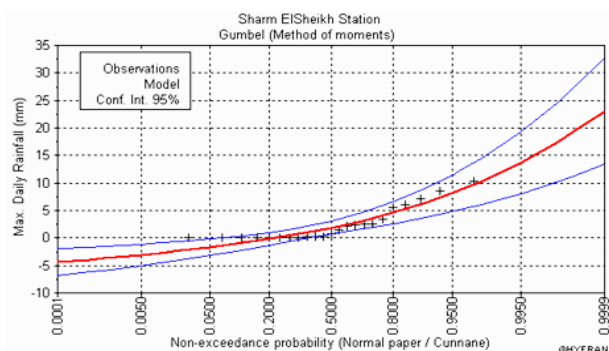
Figure 10: Statistical analysis of Sharm ElSheikh station
