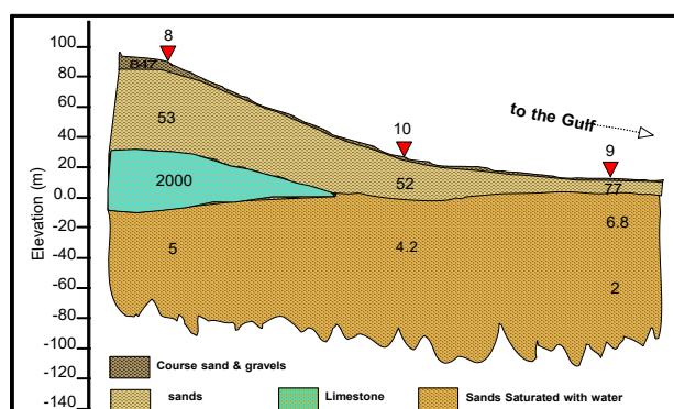
Figure 8: Geoelectric cross section B-B'
