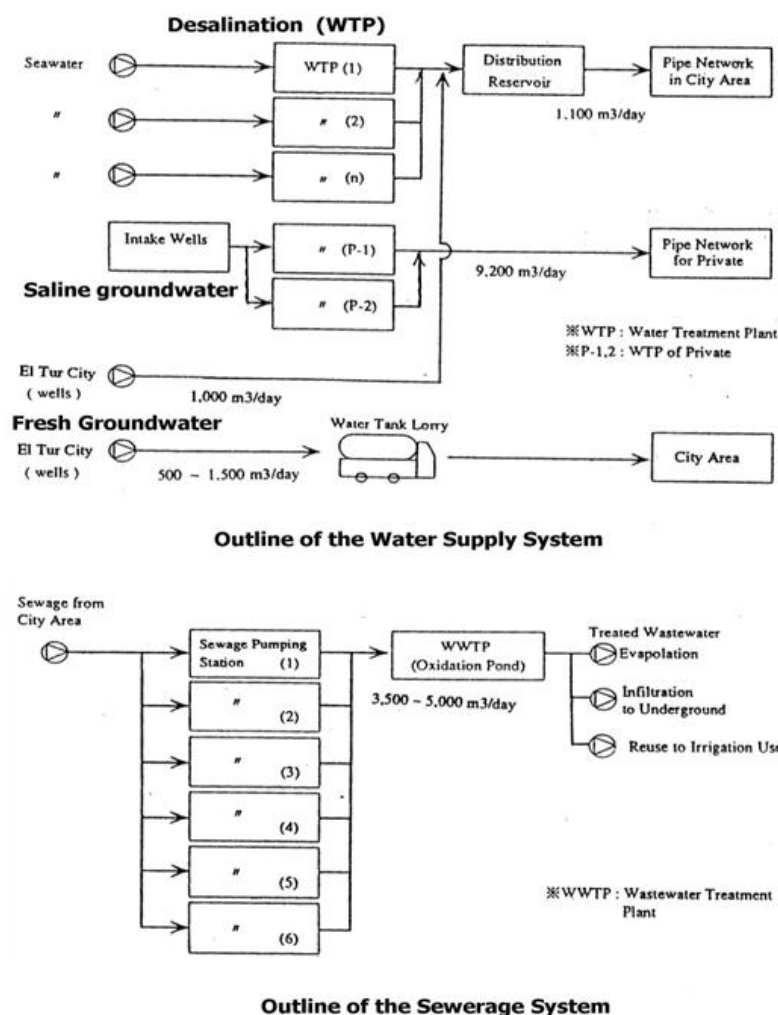
Figure 2: Outline of the status quo of water supply and sewerage system in Sharm El- Sheikh City (JICA and WRRI, 1999)
