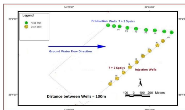
Figure 16: A flat map showing the proposed distribution of recharge and drainage well
