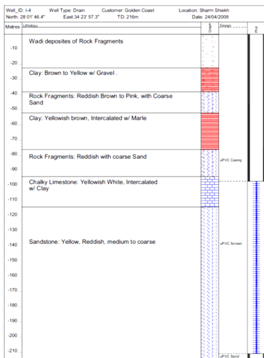
Figure 14: The subsurface lithology distribution in injection well no. I4
