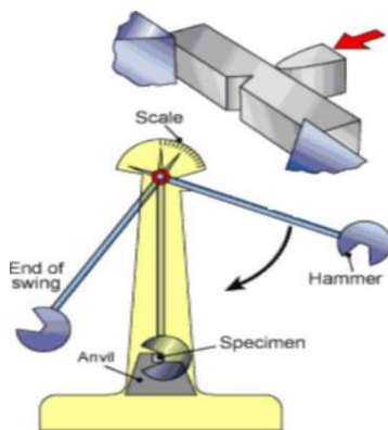
Figure 3 Charpy Test Apparatus
