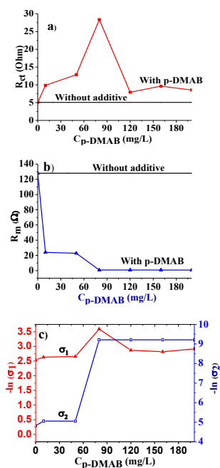
Figure 6. Dependence of kinematic parameters of redox reaction on the NAM on the concentration of p-DMAB additive in H_2SO_4 solution ( d = 1.275 \text{ g/cm}^3 ): (a) R_{ct} , (b) R_m , (c) \sigma_1 and \sigma_2 Warburg constants.
