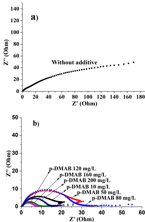
Figure 4. Nyquist-type impedance spectra on the pure lead electrode at -0.62 \text{ V} (Ag/AgCl) without (a) and with different concentrations of p-DMAB (b).
