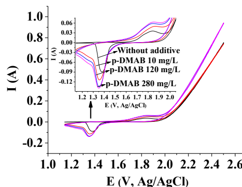
Figure 7. The cyclic voltammetry spectra of the positive active material in the H_2SO_4 solution ( d = 1.275 \text{ g/cm}^3 ) without and with different concentrations of p-DMAB. Scan rate: 50 mV/s.
