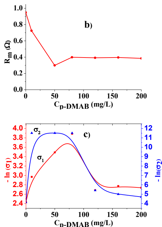
Figure 11. Dependence of kinematic parameters of redox reaction on the PAM on the concentration of p-DMAB additive in H_2SO_4 solution ( d = 1.275 \text{ g/cm}^3 ): (a) R_{ct} , (b) R_m , and (c) \sigma_1 and \sigma_2 Warburg constants.
