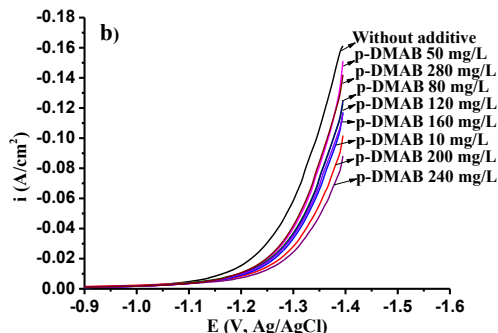
Figure 12. The linear sweep voltammograms (LCV) of Pb and Pb-3%Sb alloy in H_2SO_4 solution ( 1.275 \text{ g/cm}^3 ) without and with various concentrations of p-DMAB additive. Scan rate: 5 mV/s.
