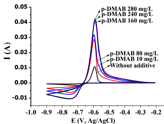
Figure 2. The cyclic voltammograms spectra of the negative active material in the \text{H}_2\text{SO}_4 solution ( d = 1.275 \text{ g/cm}^3 ) without and with different concentrations of p-DMAB. Scan rate: 50 mV/s.
