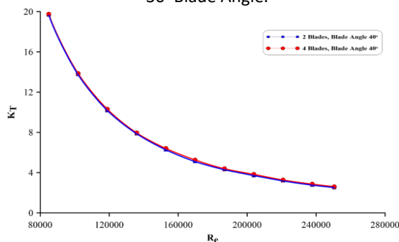
Figure 3.9 Effect of Number of Blade on Thrust Coefficient - 30° Blade Angle.
