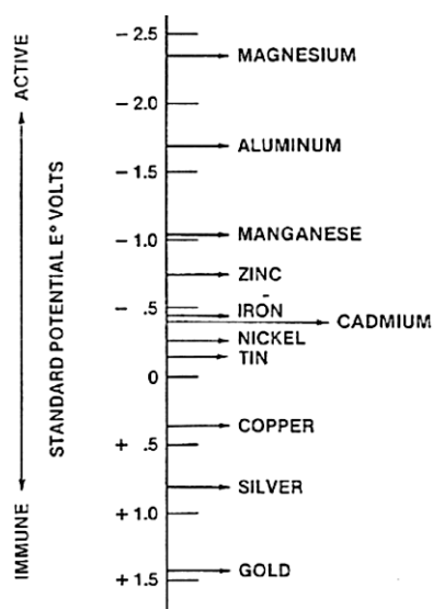
Fig. 1. Electromotive force series [1-3].
