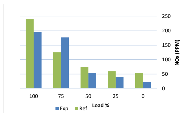
Fig.9 Validation of \text{NO}_x measurement [33]
