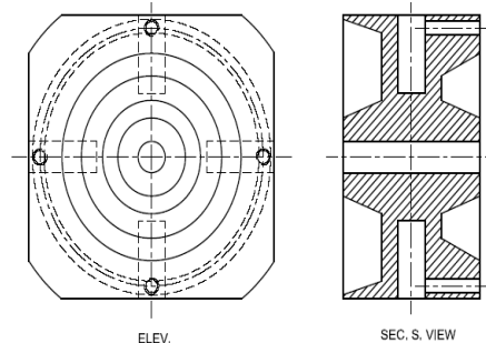
Figure 2.3 Designed hub
