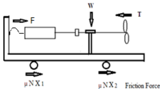
Figure 2.12 Test rig force analysis
