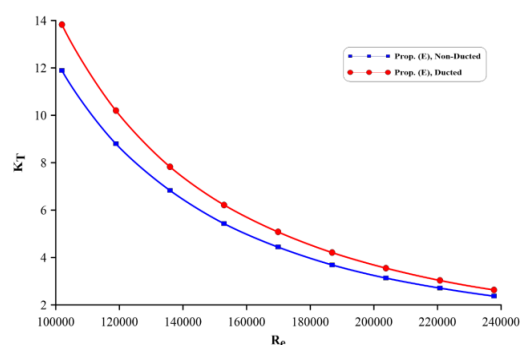
Figure 3.12 Effect of Duct on Thrust Coefficient for Propeller (E)
