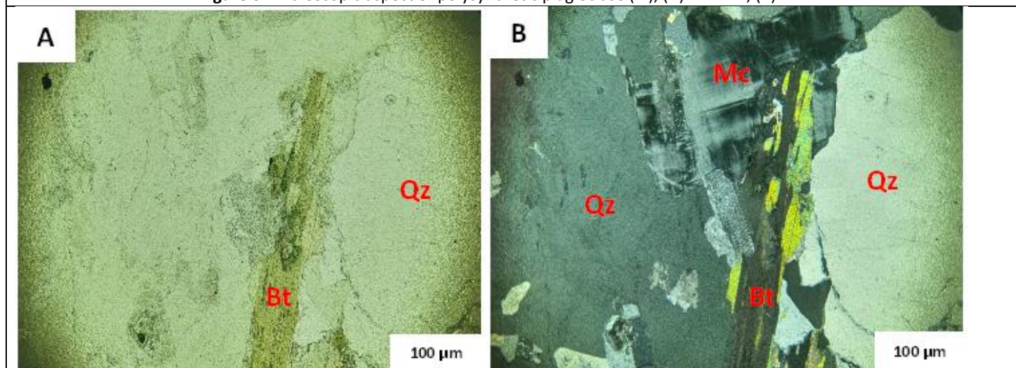
Figure 6: Microscopic aspect of polysynthetic plagioclase (Pl), (A) in LPNA, (B) in LPA
