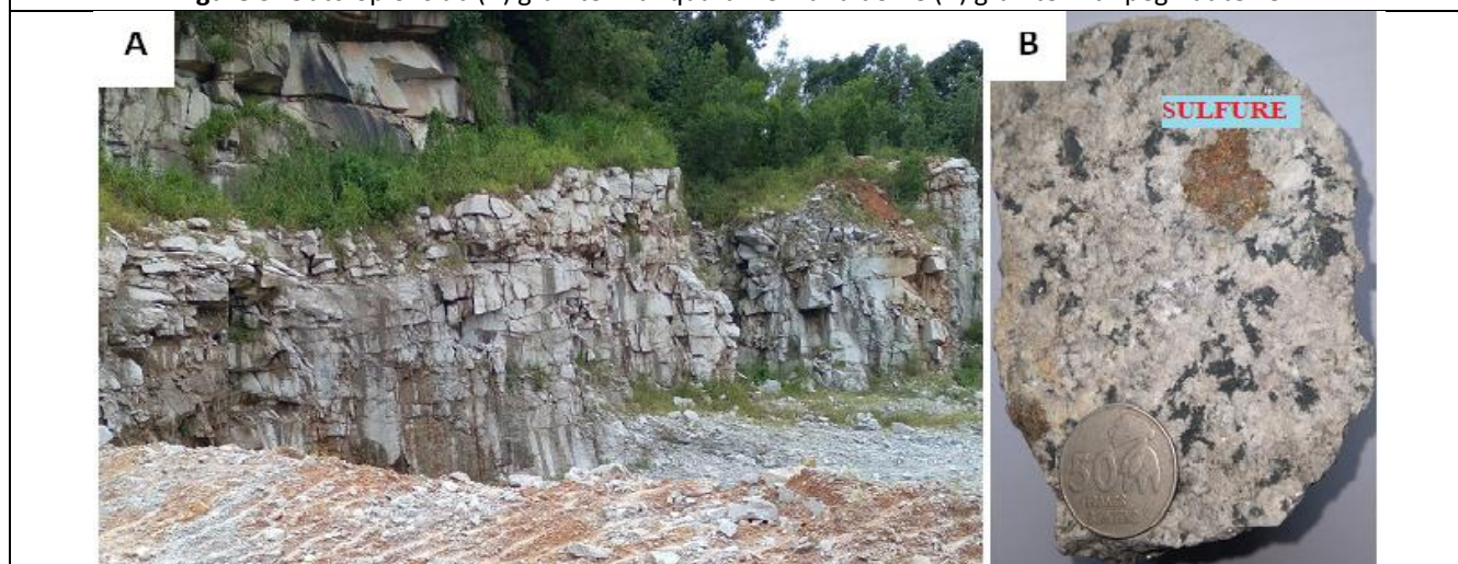
Figure 4: (A) Macroscopic appearance of SOMIAG quarry granites, (B) Inclusion of sulphide in a granite sample from the SOMIAG quarry
