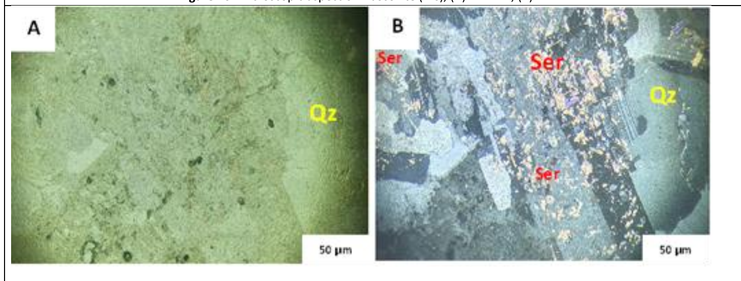
Figure 11: Microscopic appearance of sericite (Ser), (A) in LPNA, (B) in LPA
