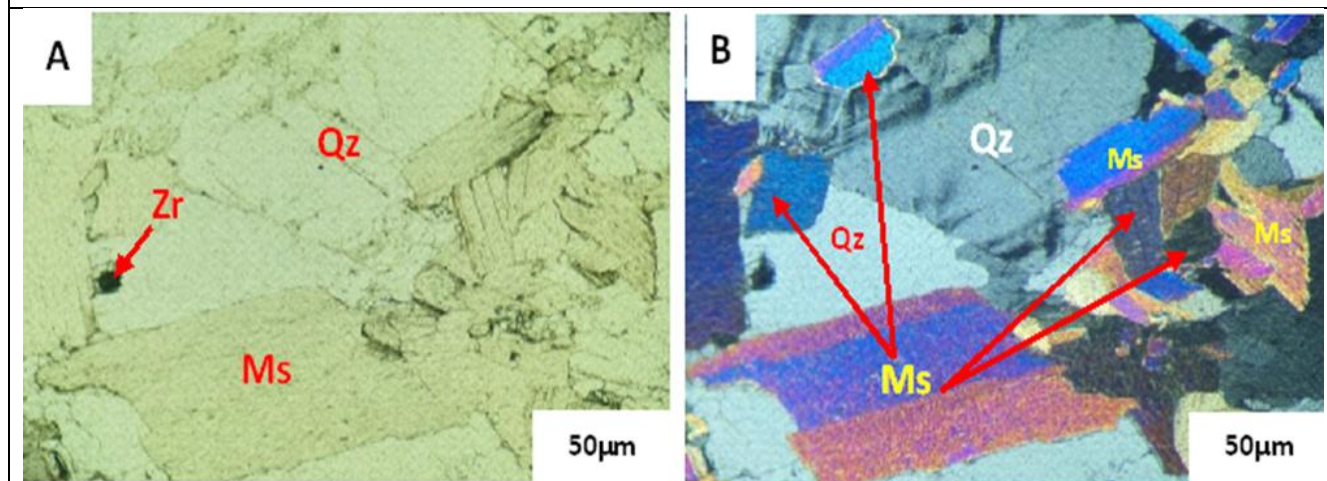
Figure 20: Microscopic aspect of biotite (Bt), (A) in LPNA, (B) in LP
