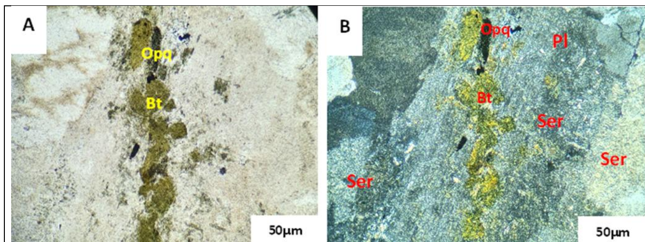
Figure 19: Microscopic appearance of sericite (Ser), (A) in LPNA, (B) in LP
