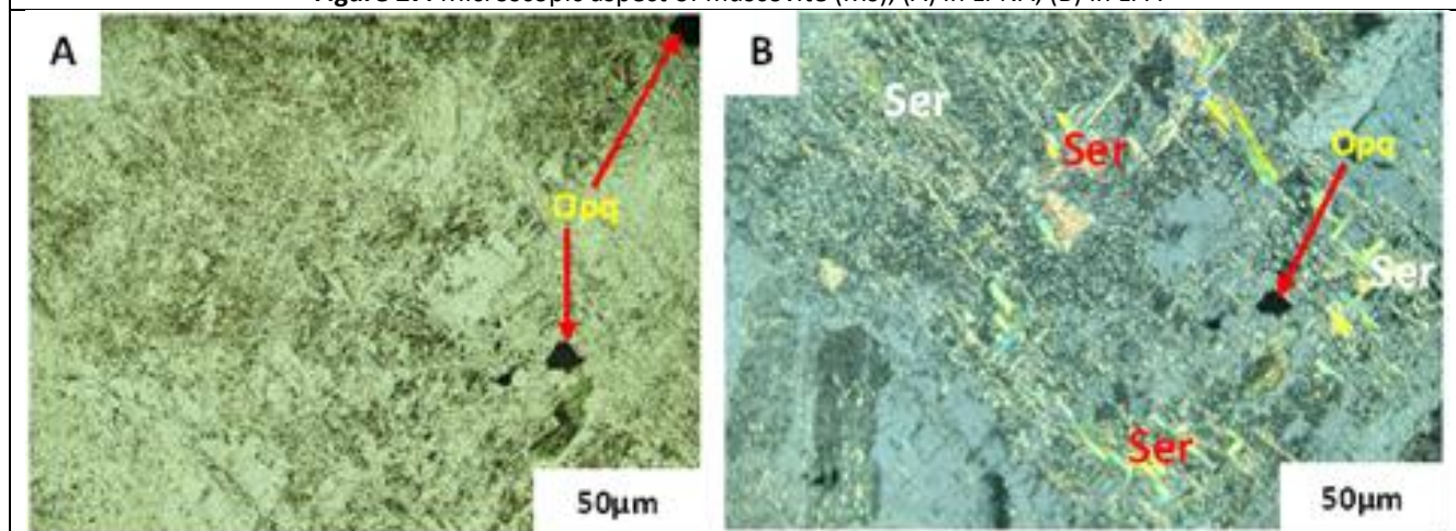
Figure 28: Microscopic appearance of sericite (Ser), (A) in LPNA, (B) in LPA
