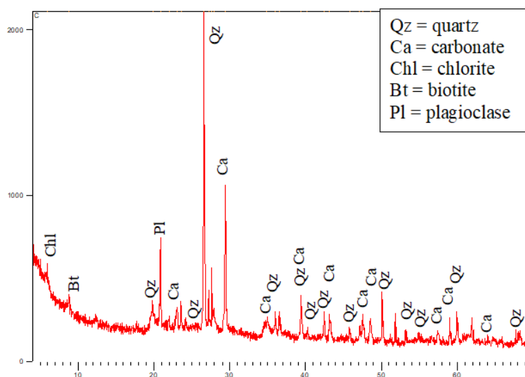
Figure 14: SOMIAG quarry sample diffractogram
