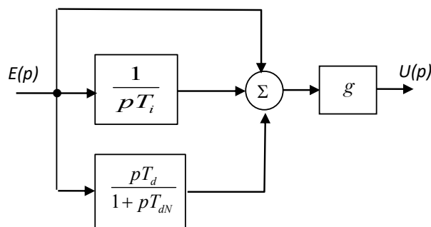
Fig. 4 Functional scheme for PID controller
