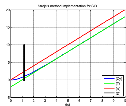
(b) Strejc's method for SIB
